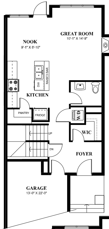
9' MAIN FLOOR 650 sq. ft.
